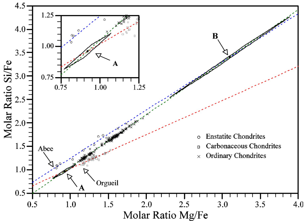
Figure 1 Molar (atom) ratios of Mg/Fe and Si/Fe from analytical data on 10 enstatite chondrites, 39 carbonaceous chondrites, and 157 ordinary chondrites. Data from Baedeker & Wasson (1975), Jarosewich (1990), Wiik (1969). Members of each chondrite class data set scatter about a unique, linear regression line indicated by dashes. The locations of the volatile-rich Orgueil carbonaceous chondrite and the volatile-rich Abee enstatite chondrite are indicated. Line intersections A and B are designated, respectively, primitive and planetary components. Error estimates of points A and B are indicated by solid-line parallelograms formed from the intersections of the standard errors of the respective linear regression lines. Inset shows in expanded detail the standard error parallelogram of point A.
